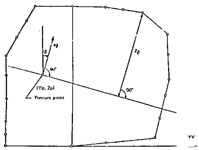
Figure 4.2—Determination of internal pressure heads
